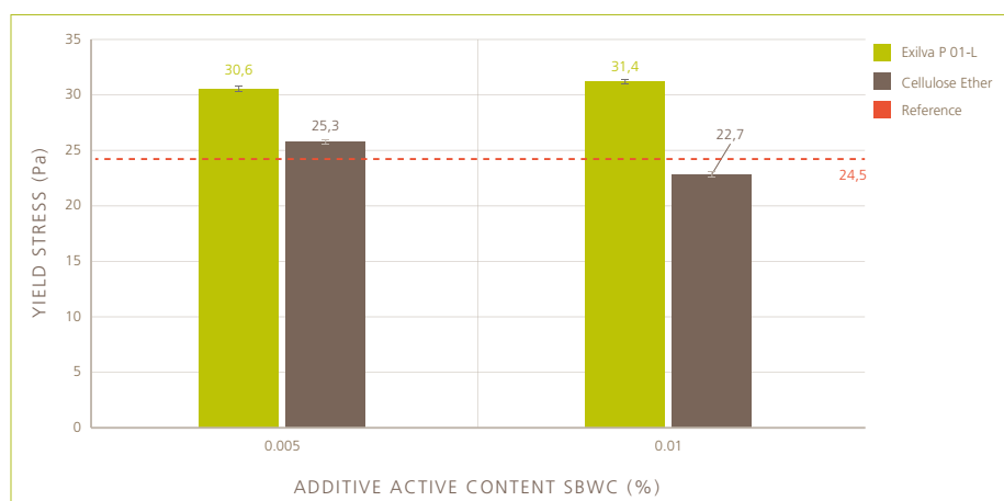
FIGURE 1: Yield Stress Values for the Cement Pastes Tested.
